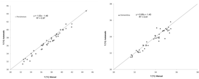
Fig. 4 Comparison of manual and automatic calculation procedures of average canopy temperatures ( T_c ) for a representative day where the coefficient of determination ( r^2 ) and the linear regression equations are shown. A) Persimmon (DOY 204). B) CN (DOY 215). The solid lines in each figure represent the 1:1 relationship.
